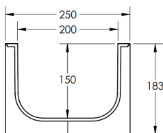
200MM PROFILE
