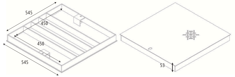
SERIES 450 GALVANISED CHECKER PLATE COVER
