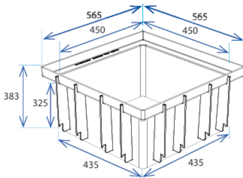
SERIES 450 SHALLOW STORMWATER PIT
