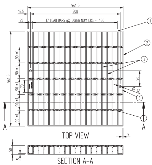
21041 GALVANISED GRATE
