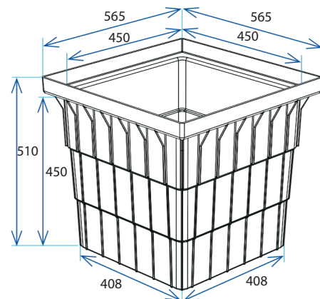
SERIES 450 DEEP STORMWATER PIT
