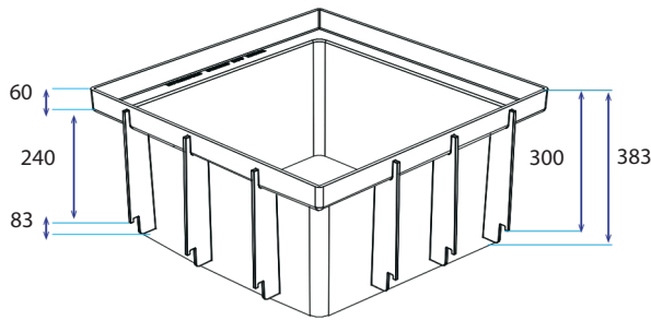
SERIES 450 RISER
