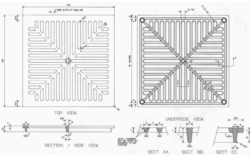
SERIES 300 ALUMINIUM GRATE
