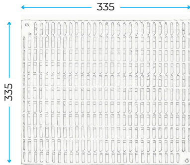
SERIES 300 GALVANISED GRATE
