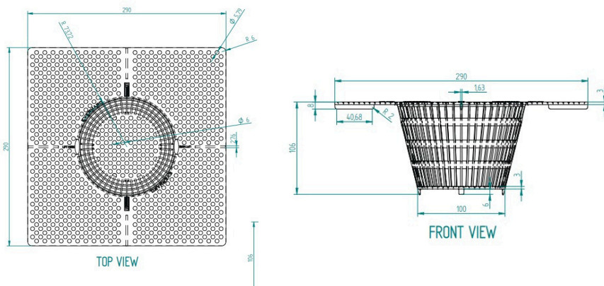
SERIES 300 STORMWATER PIT LEAF BASKET
