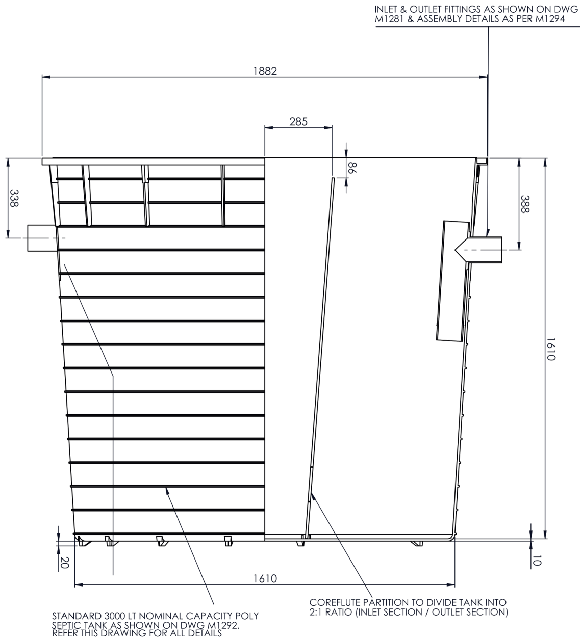
2500L SEPTIC TANK
