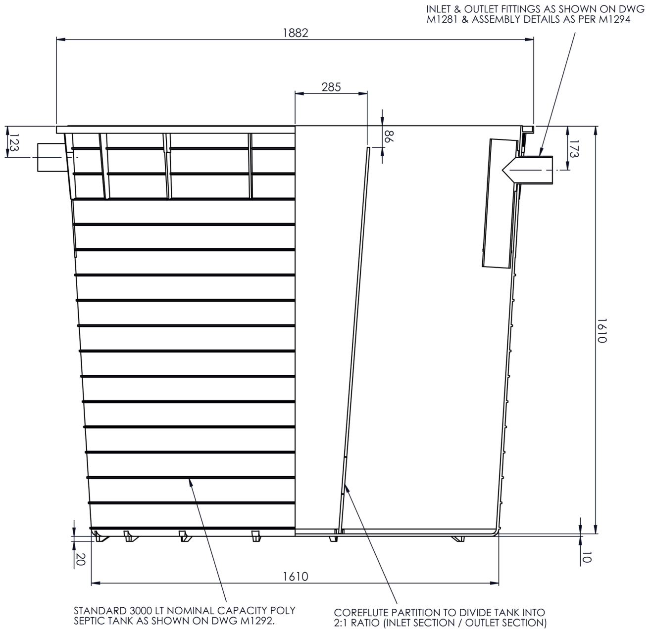
3000L SEPTIC TANK
